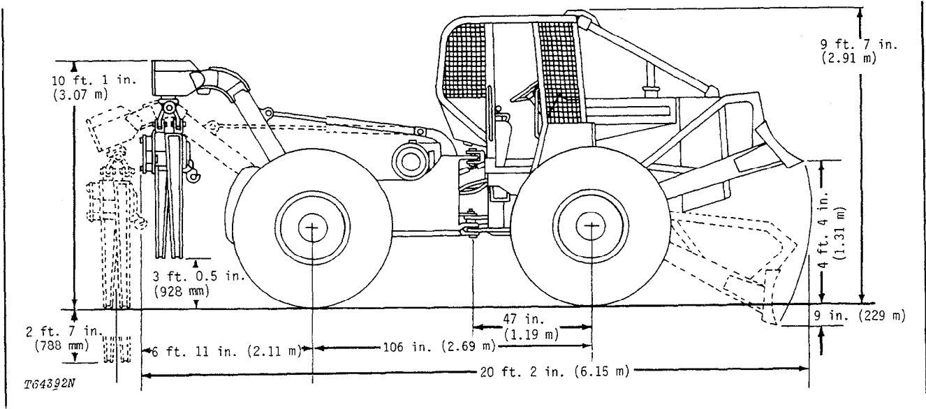
Side view dimensions are for skidder equipped with 23.1-26 tires, grapple open.
